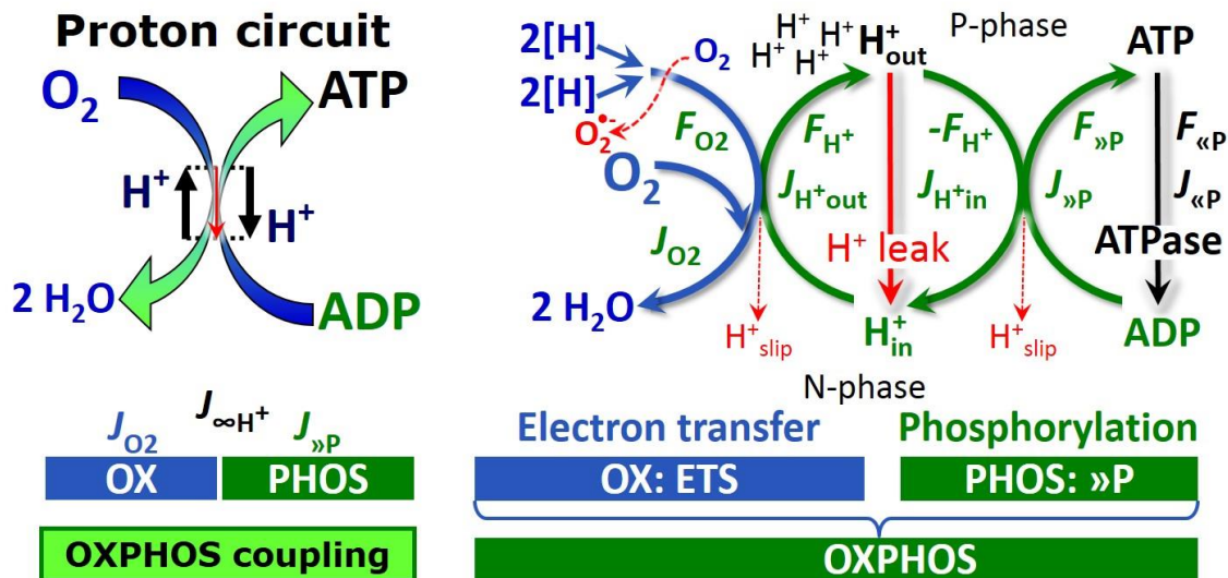
Fig. 2. The proton circuit and coupling in oxidative phosphorylation (OXPHOS). Oxygen flux, J_{\text{O}_2} , is coupled to the phosphorylation of ADP to ATP, J_{\gg P} , by the proton pumps of the electron transfer system, ETS, pushing the outward proton flux, J_{\text{H}^+\text{out}} , generating the output protonmotive force, F_{\text{H}^+} . ATP synthase is driven by the input protonmotive force, -F_{\text{H}^+} , and inward proton flux, J_{\text{H}^+\text{in}} , to phosphorylate ADP to ATP. 2[\text{H}] indicates the reduced hydrogen equivalents of fuel substrates that provide the
