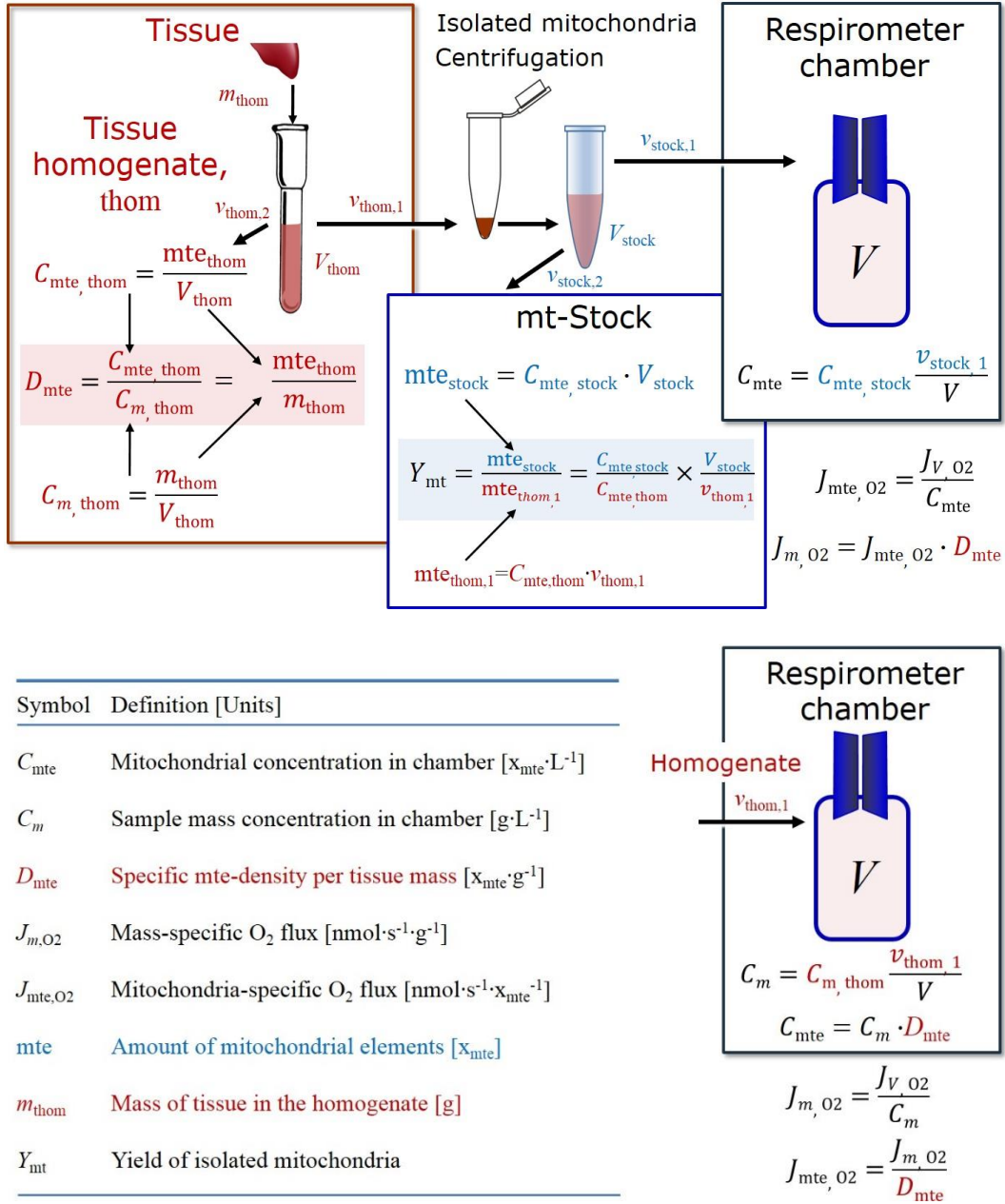
Fig. 8. Normalization of volume specific flux of isolated mitochondria and tissue homogenate. A: Mitochondrial yield, Y_{mt} , in preparation of isolated mitochondria. v_{thom,1} and v_{stock,1} are the volumes transferred from the total volume, V_{thom} and V_{stock} , respectively. mte_{thom,1} is the amount of mitochondrial elements in volume v_{thom,1} used for isolation. B: In respirometry with homogenate, v_{thom,1} is transferred directly into the respirometer chamber. See Table 6 for further explanation of symbols.
