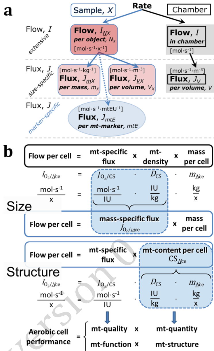
Figure 5. Flow and flux, and normalization in structure-function analysis
