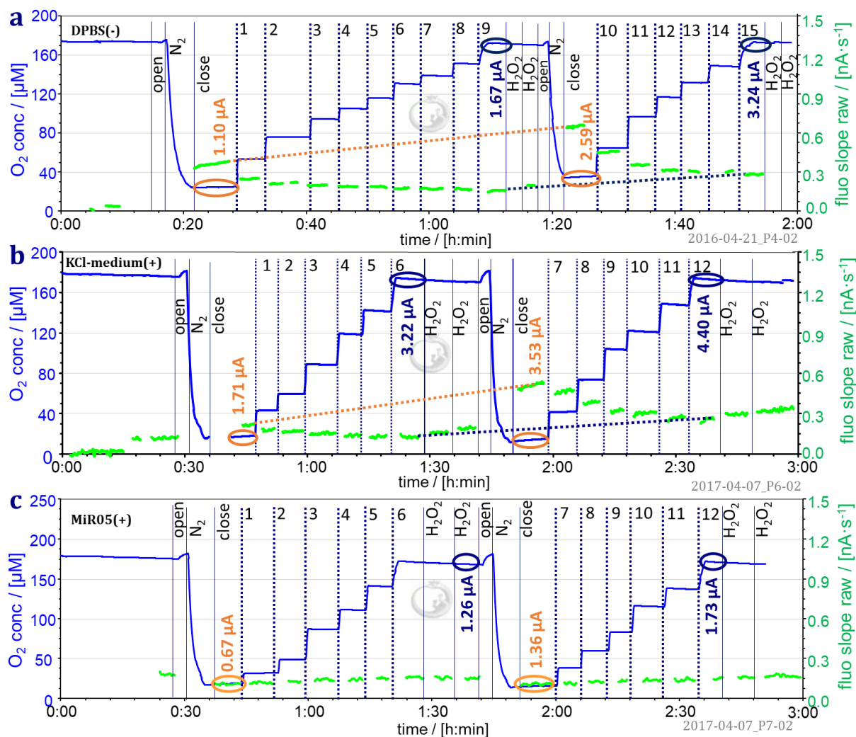
Figure 4. Oxygen dependence of the background fluorescence slope in the Amplex™ UltraRed assay. (a) DPBS(-); (b) KCl-medium(+); (c) MiR05(+) (see Figure 5c). Blue plots: O_2 concentration ( \mu\text{M} ) was decreased with N_2 in the gas phase followed by increase of the O_2 concentration in several steps (1 to 15 and 1 to 12). Green plots: background fluorescence slope (raw) \text{nA}\cdot\text{s}^{-1} . The background fluorescence intensity (raw) ( \mu\text{A} ) is shown at low O_2 concentration (values in orange) and at high O_2 concentration (values in blue). Dotted orange lines: pronounced increase of the apparent H_2O_2 flux at low O_2 concentration as a function of the fluorescence intensity ( \mu\text{A} ) (values in orange); dotted blue lines: less pronounced increase of the apparent H_2O_2 flux at high O_2 concentration as a function of fluorescence intensity (values in blue).
