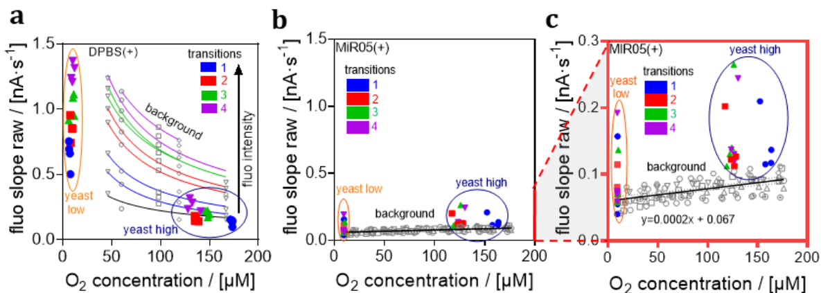
Figure 6. Fluorescence slope (apparent \text{H}_2\text{O}_2 flux with or without yeast) as a function of oxygen concentration in DPBS and MiR05. Non-calibrated fluorescence slope [ \text{nA}\cdot\text{s}^{-1} ] in background (without yeast; open grey symbols) and in the presence of yeast in the reoxygenation cycles with transitions from high to low \text{O}_2 concentrations (closed symbols; enclosed by blue and orange outlines, respectively). Identical colors of symbols indicate technical repeats ( n=4 ). Different colors of symbols distinguish the first to fourth transitions (1 to 4). (a) DPBS(+) background (from Figure 5a). Lines are fitted by nonlinear regression through data points at constant fluorescence signal; r^2=0.96-0.99 . Different colors of lines reflect the pattern of fluorescence intensity measured in the reoxygenation cycles with yeast (from Figure 2d; peak fluorescence at low \text{O}_2 concentrations). (b) MiR05(+) background (from Figure 1e). Line is fitted by linear regression; r^2=0.80 . (c) Zoom into panel b .
