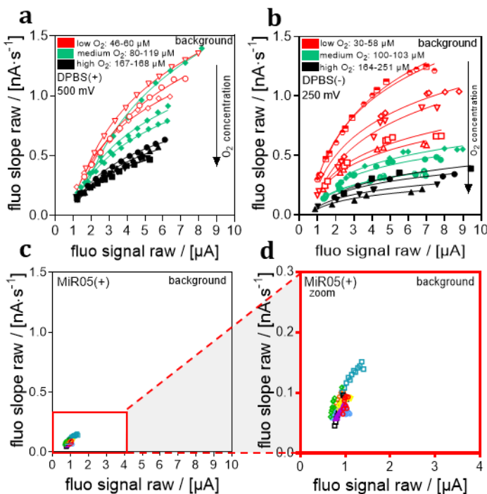
Figure 5. Oxygen dependence of the background fluorescence slope (apparent H_2O_2 flux without yeast) as a function of fluorescence signal [ \mu A ] (proportional to fluorescence intensity) in DPBS and MiR05. Background fluorescence slope (raw) [ nA \cdot s^{-1} ] as a function of fluorescence signal. (a) DPBS(+), excitation light intensity 500 mV; ten different O_2k -chambers ( n=10 , five O_2k ). Lines are fitted by nonlinear regression; r^2=0.95-0.99 . (b) DPBS(-) without DTPA, excitation light intensity 250 mV; 14 different O_2k -chambers ( n=14 , seven O_2k ); r^2=0.95-0.99 . For DPBS, colors indicate
